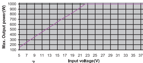
1030 Charger: MAX. OUTPUT POWER vs. INPUT VOLTAGE
