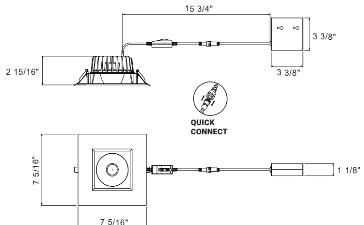
PRODUCT DIMENSIONS
