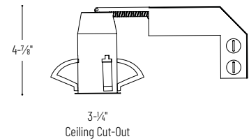
NHRIOIC-28LE4 2" Iolite IC Air-Tight Remodel Housing
