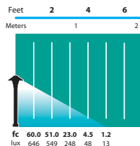
AL-01-SM Half Spread Photometrics 10 ft. (3.0m) diameter
