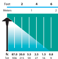
AL-01 Half Spread Photometrics 12 ft. (3.7m) diameter
