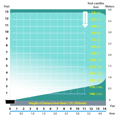
SL-08-FL-9 Half Spread Photometrics (9w)
