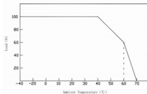
Derating Curve
