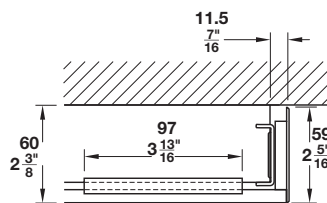
For aluminum panel, aluminum lateral cover
