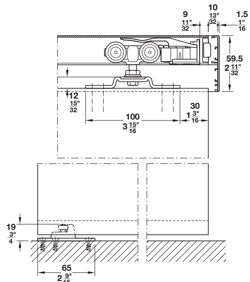
Trolley hanger, track stopper and floor guide
