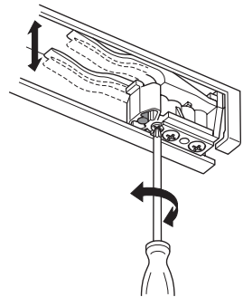
Stopper with adjustable locking force
