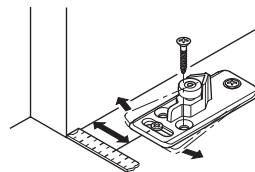
Side adjustable floor guide
