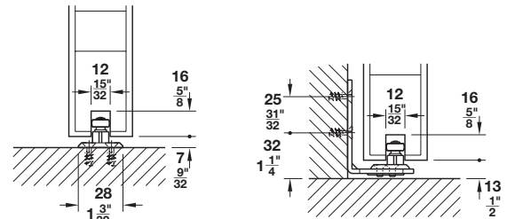
Standard floor guide
