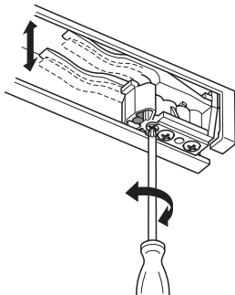
Stopper with adjustable locking force
