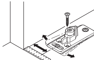
Side adjustable floor guide
