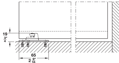
Trolley hanger, track stopper and floor guide Clip part for cover caps and panels
