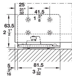
Floor guide with wall mounting bracket
