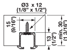
Upper track, for gluing into groove
