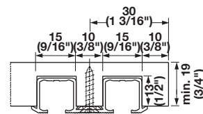
Upper track, with rotating fasteners
