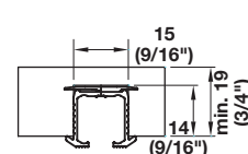
Upper track, with rotating fasteners
