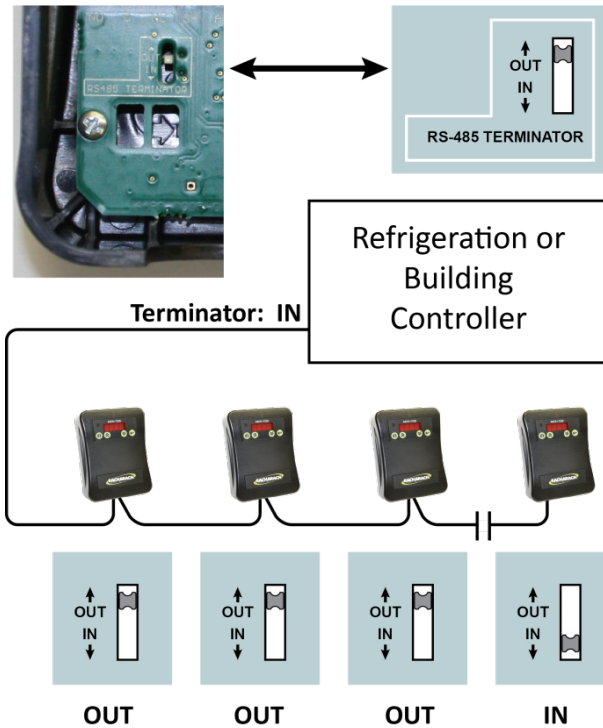
Figure 13. Setting Network Termination Resistors
