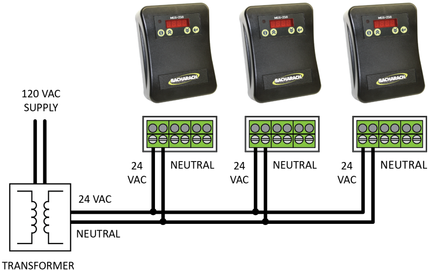
Figure 9. Maintaining Neutral Polarity
