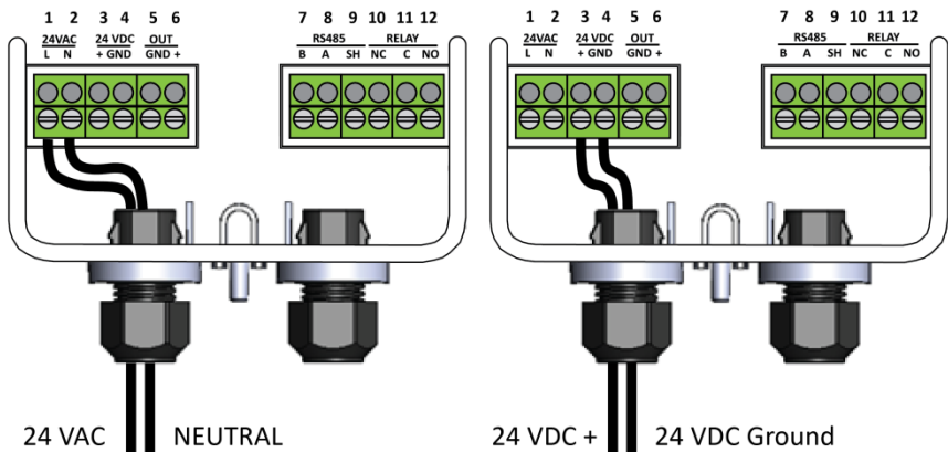
Figure 8. Supply Power Wiring Options
