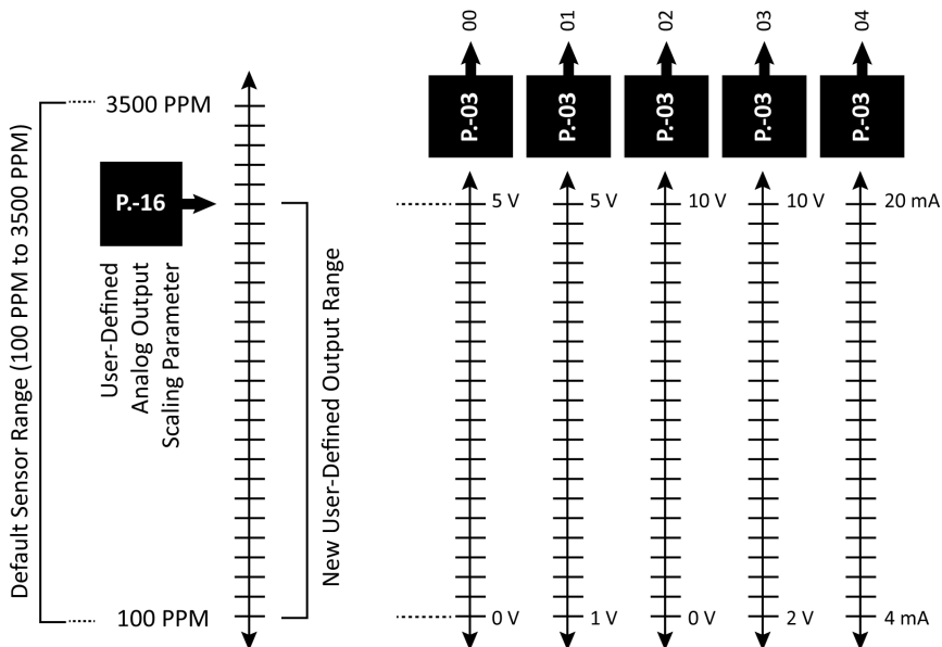
Figure 15. Analog Output Scaling Options
