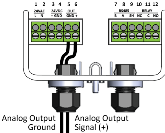
Figure 10. Analog Output Wiring
