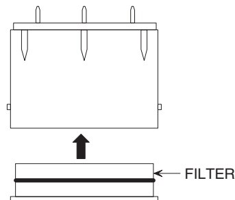
Figure 4-4. CO-LO, CO-HI, and NO Sensor Filter Replacement
