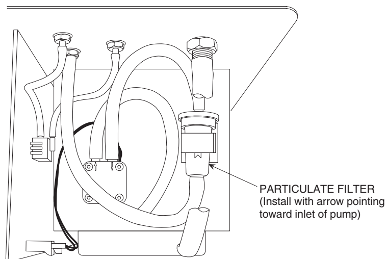
Figure 4-5. Replacing the Internal Particulate Filter
