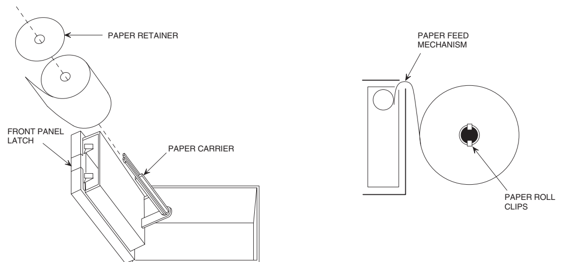
Figure 4-2. Installing Printer Paper
