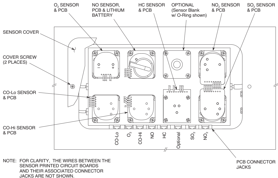
Figure 4-3. Sensor Compartment
