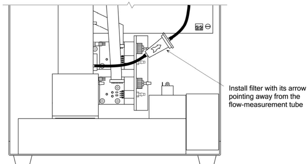
Figure 5-3. Leak-Gas Filter
