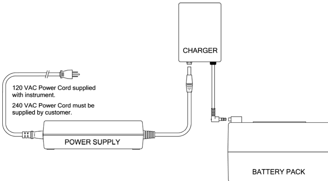
Figure 5-1. Charging the Battery Pack
