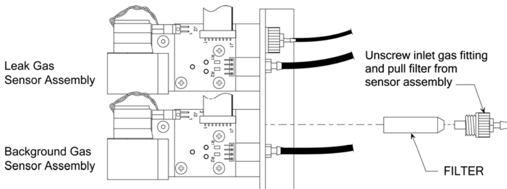
Figure 5-4. Leak Gas & Background Gas Sensor Filter Replacement
