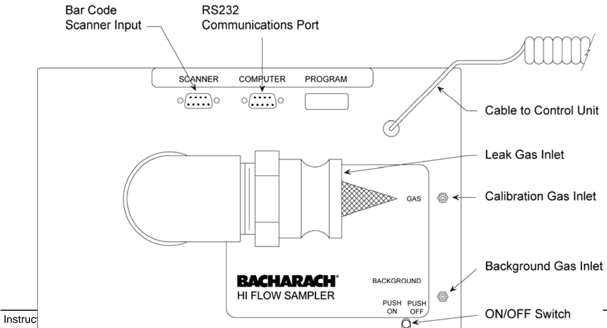
Figure 1-2. Top Panel Connections
