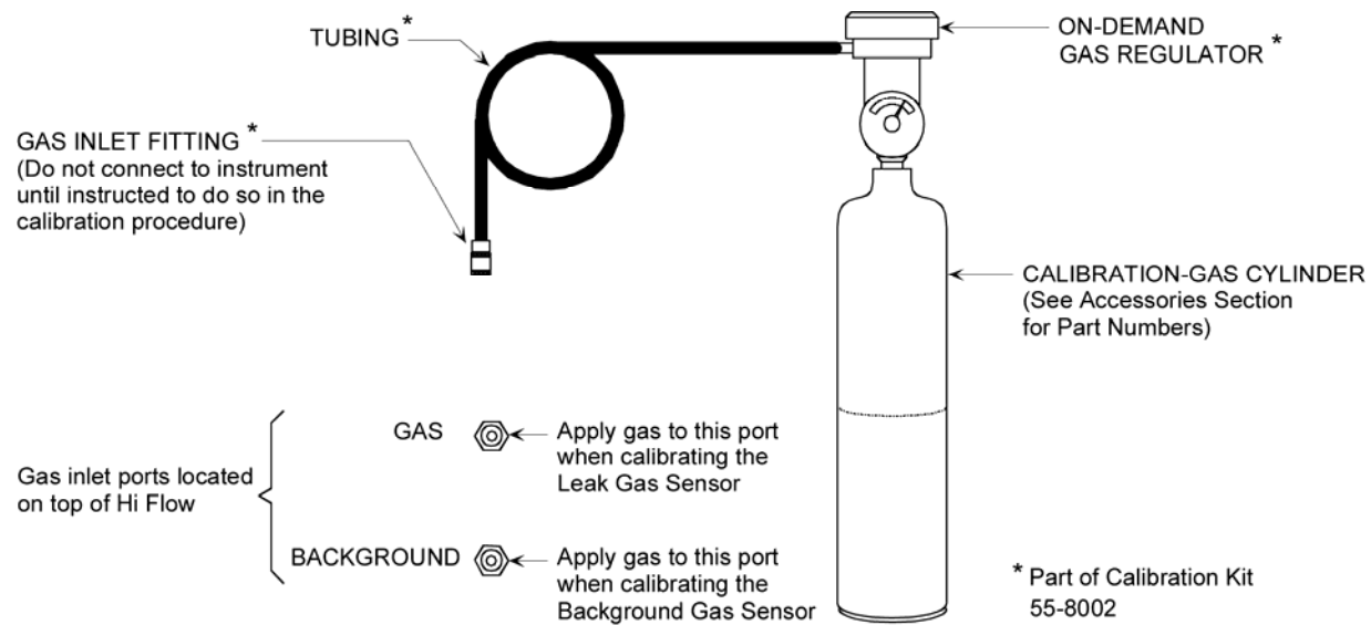
Figure 4-1. Calibration Equipment Setup
