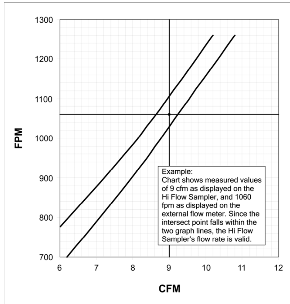
Figure 5-8. Flow Rate Validation Graph
