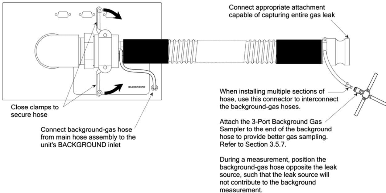
Figure 3-2. Hose and Attachment Connections
