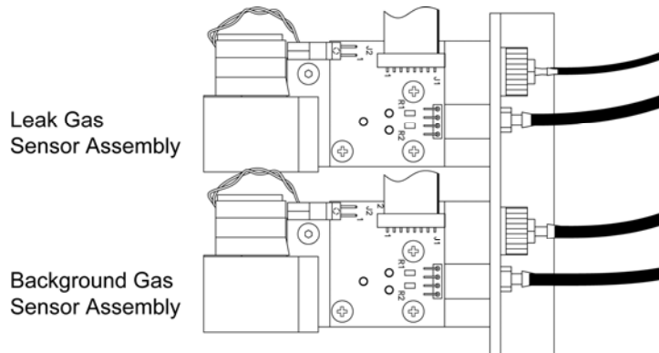
Figure 5-5. Leak-Gas & Background Gas Sensor Assemblies
