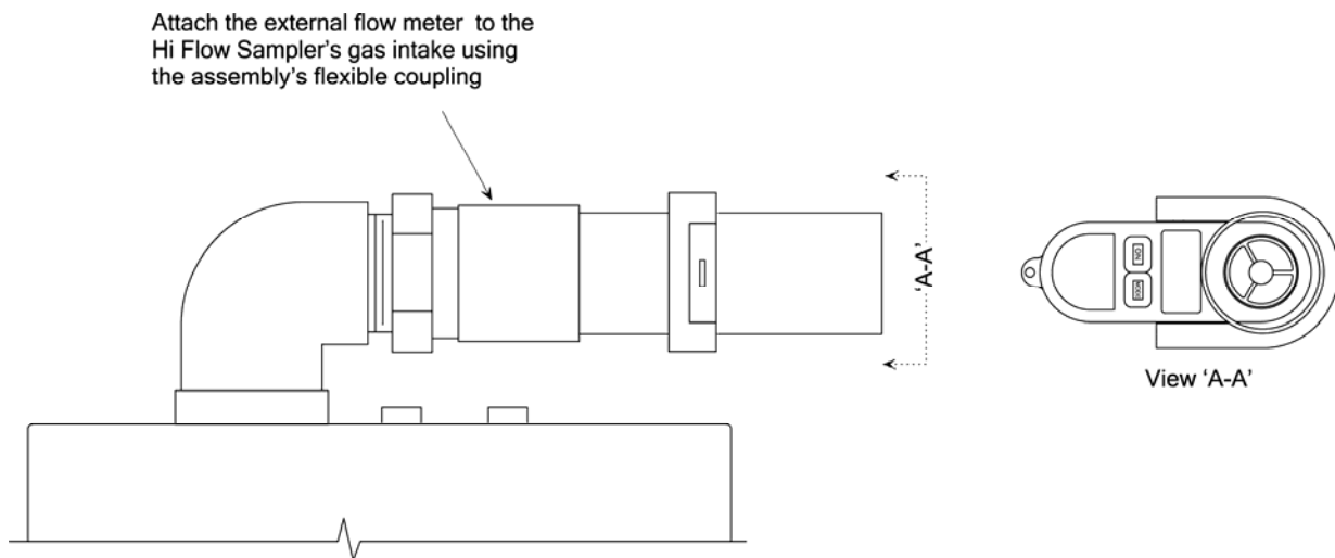
Figure 5-7. Flow Meter Installation
