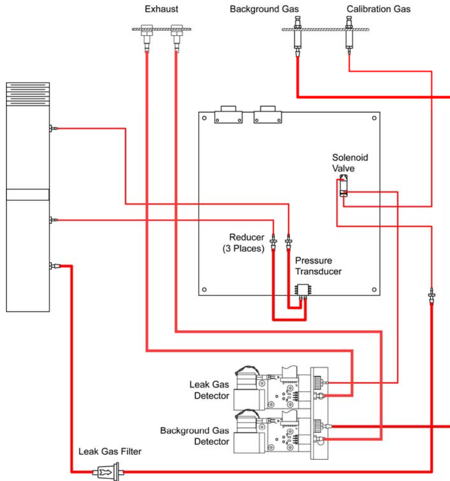
Figure 5-10. Plumbing Diagram
