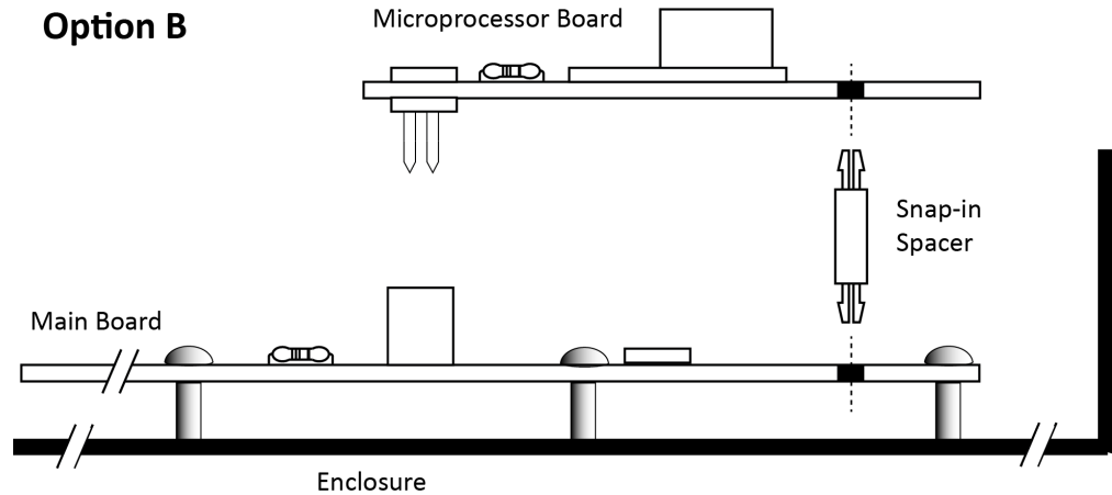
Figure 4. Option B Installation
