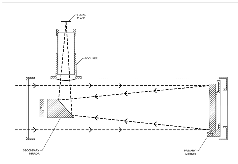
Figure 3-1 Cutaway view of the light path of the Newtonian optical design.
