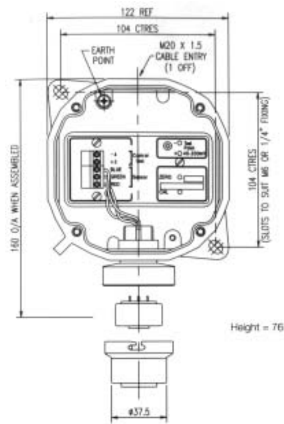
Diagram 1: TXgard-IS is fitted with bayonet type sensor housing
