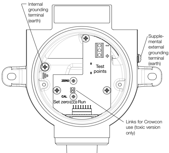
Diagram 6: Xgard Type 2 PCB layout (Shown with PCB cover removed).
