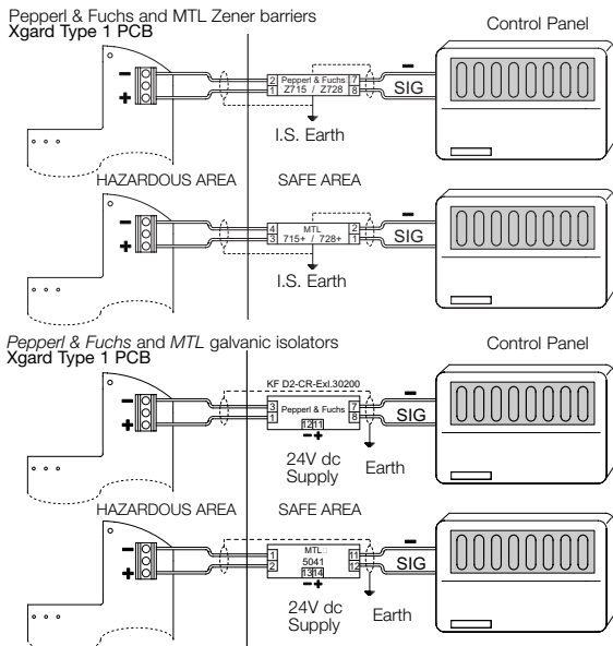
Diagram 5: Xgard Type 1 electrical connections
