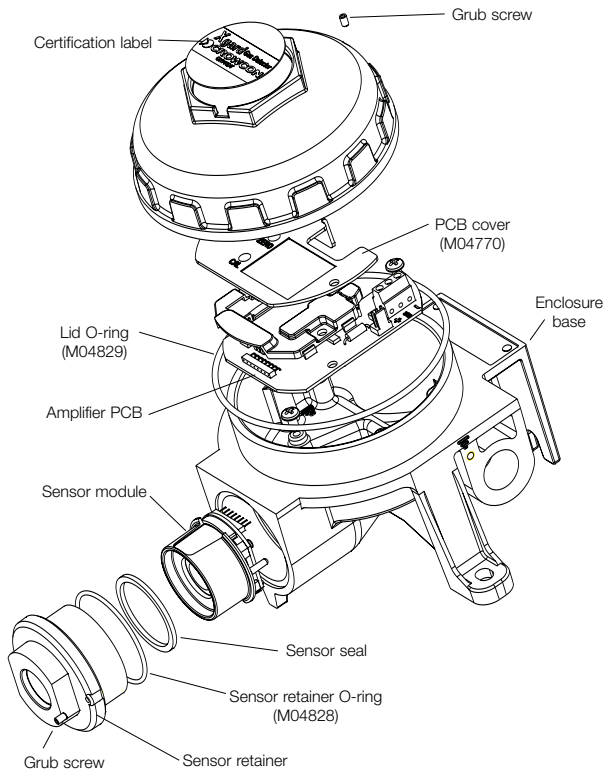
Diagram 3: Xgard exploded view (part numbers shown in brackets where applicable. For part numbers not shown, see Spares and Accessories on page 59)
