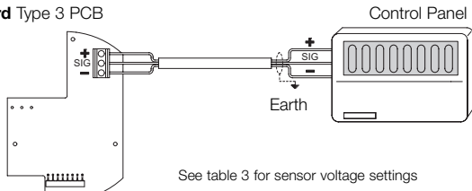
Diagram 9: Xgard Type 3 electrical connections
