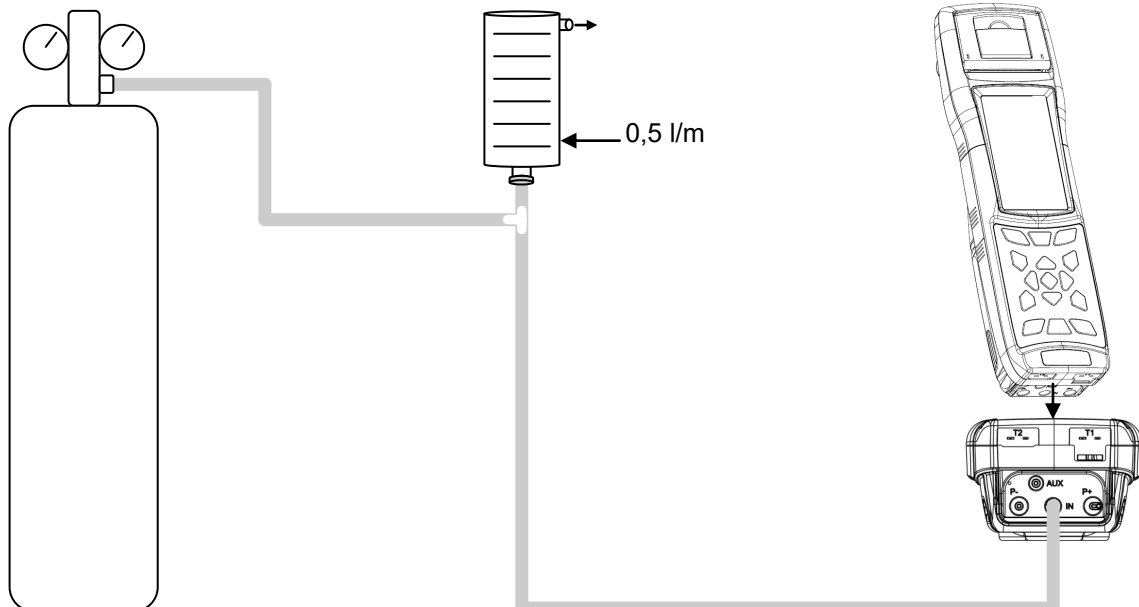
GAS CYLINDER
