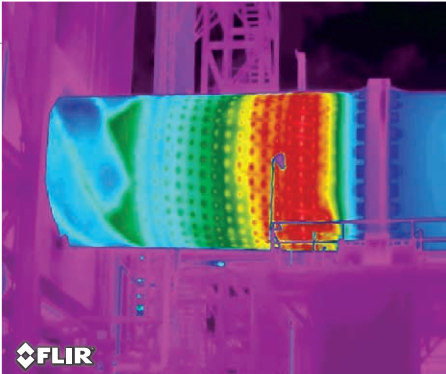
Rotary kiln showing elevated skin temperature.
