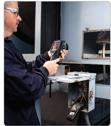
FLIR CM78 transmits real-time electrical measurements to FLIR IR cameras via METERLiNK
