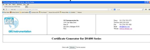
certificate_generator_v00.78.html
