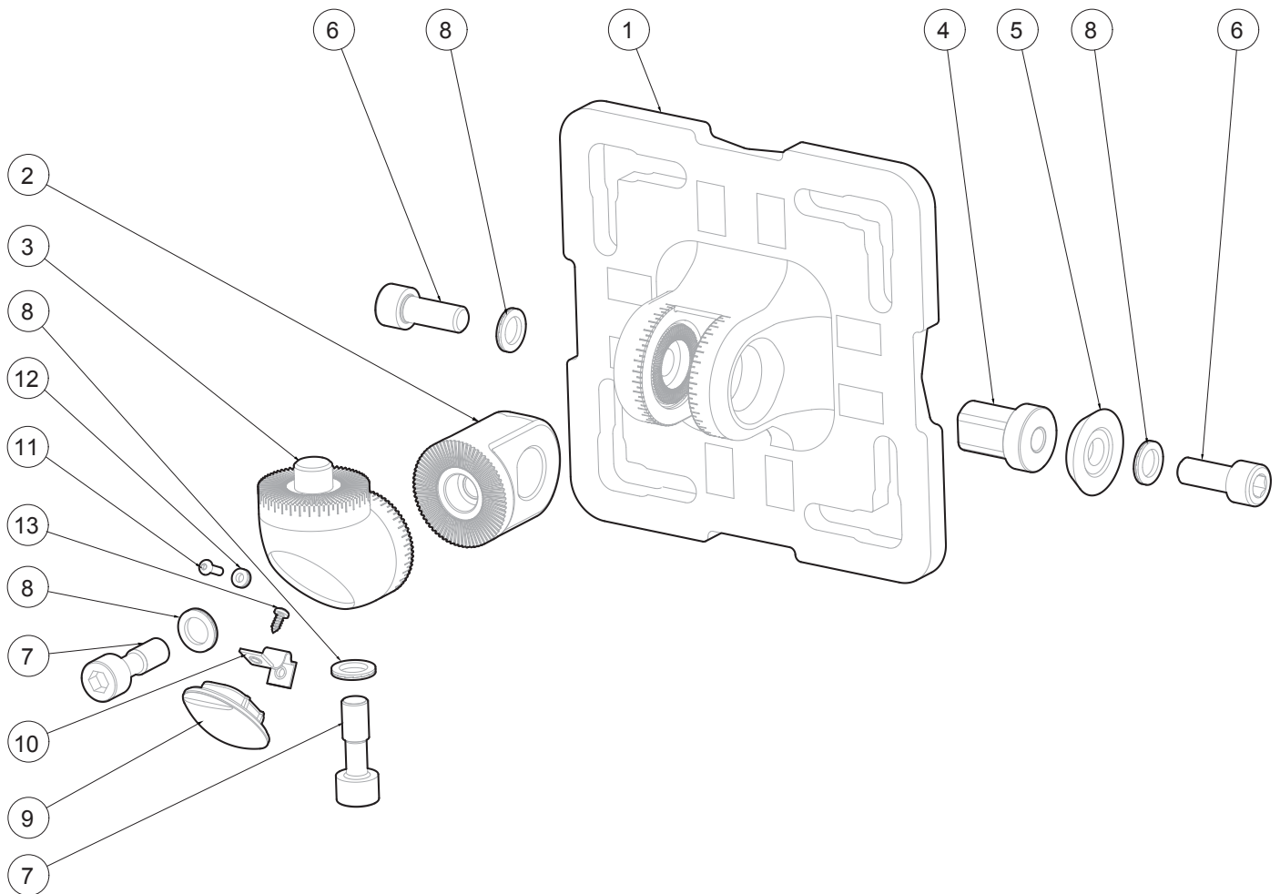
Figure 10. Standard Adjustable Mounting Bracket exploded view
