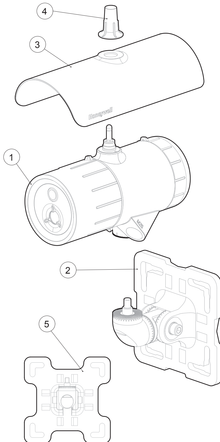
Figure 8. Searchzone Sonik general view
