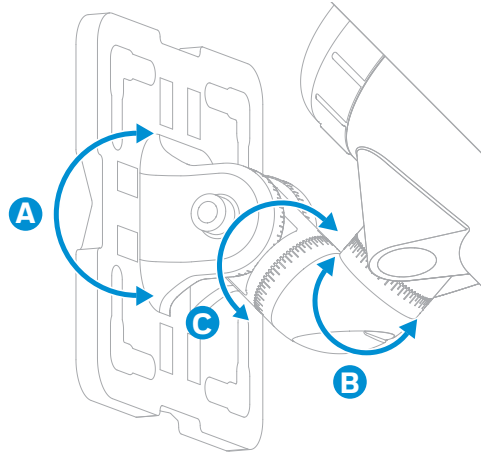
Figure 6. Adjustment ranges
