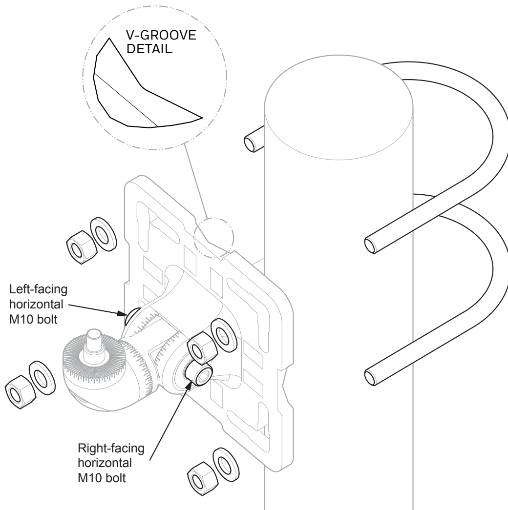
Figure 11. Standard Adjustable Mounting Bracket fitment to pole with U-bolts
