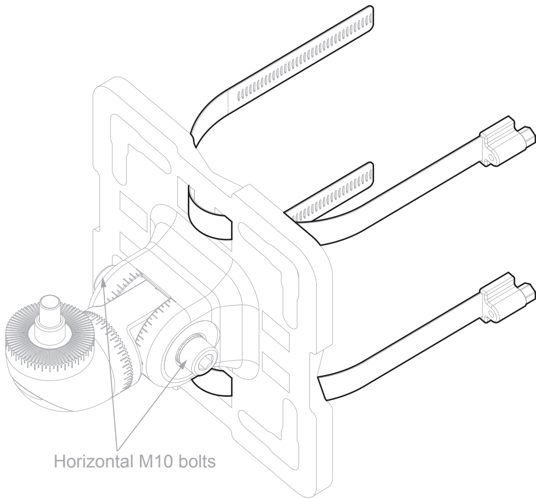
Figure 12. Standard Adjustable Mounting Bracket fitment using Worm Drive Clips
