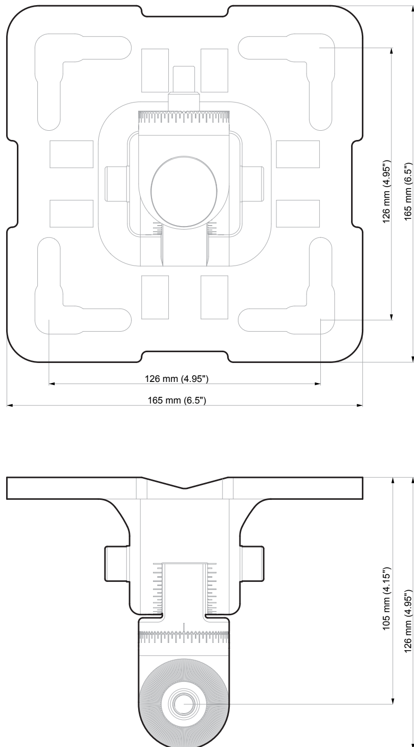
Figure 9. Standard Adjustable Mounting Bracket general view and dimensions
