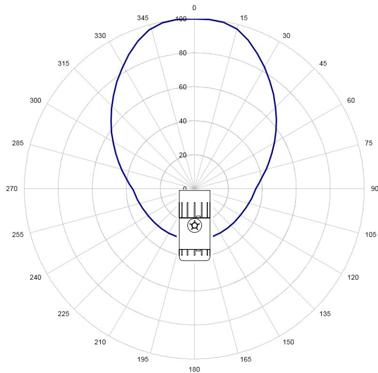
Figure 4. Angular Field of Coverage in Focus Mode (% of Range)
