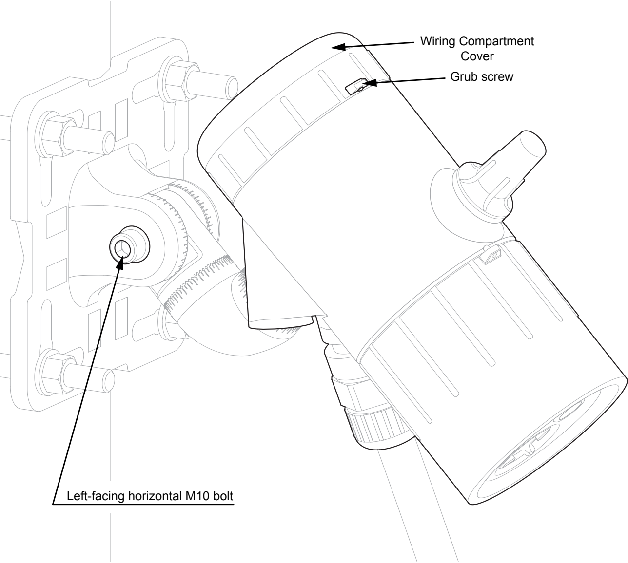
Figure 19. Example position of 45°
