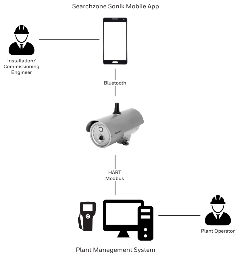
Figure 7. Searchzone Sonik communication diagram
