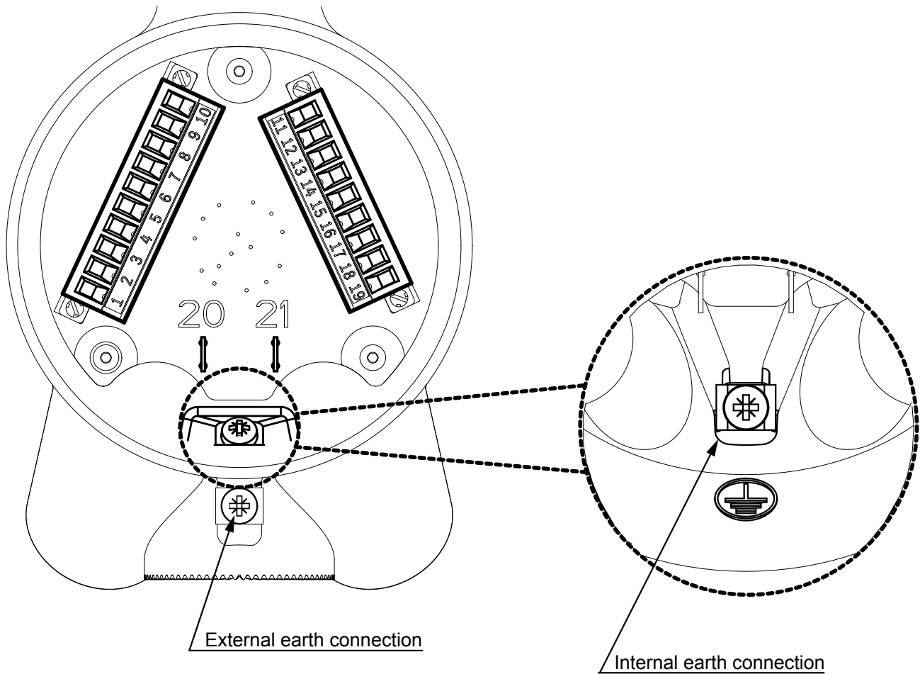
Figure 22. Terminal Wiring Compartment
