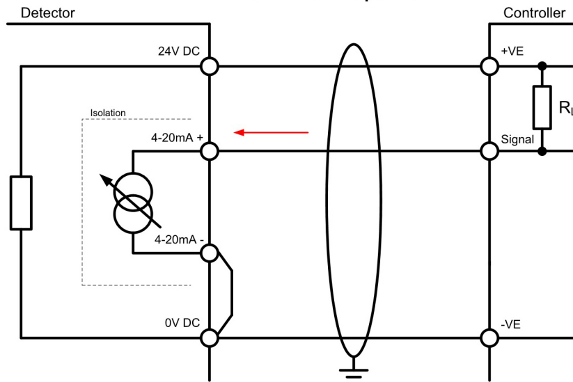
Figure 24. mA loop configuration as current sink
