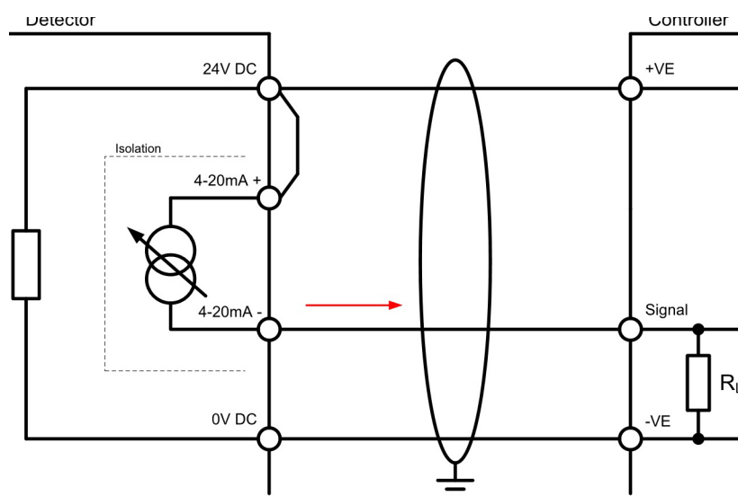
Figure 23. mA loop configuration as current source
