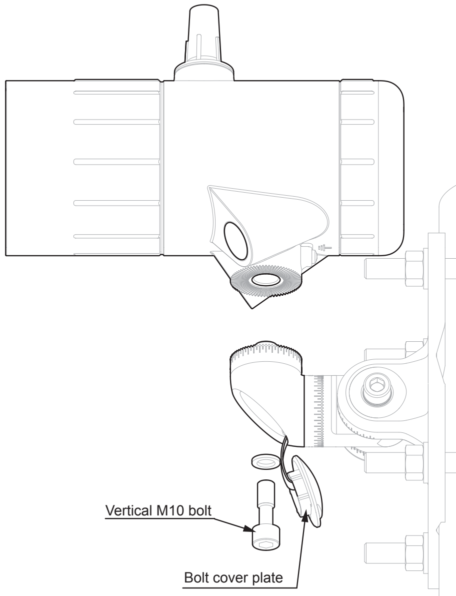
Figure 16. Detector attachment
