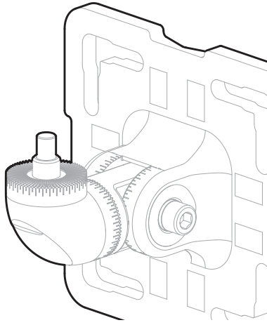
Figure 5. Standard Adjustable Mounting Bracket
