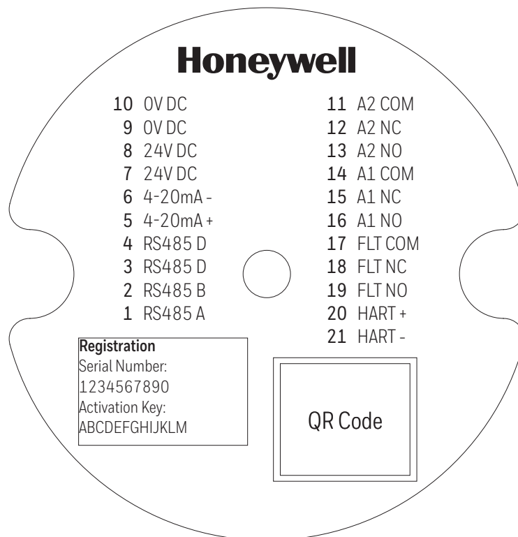
Figure 21. Terminal Connector Label
