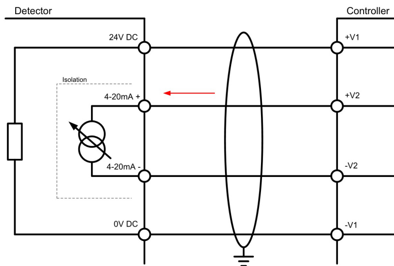
Figure 25. mA loop configuration as isolated output
