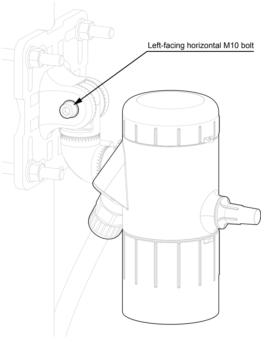
Figure 17. Set the vertical position of Detector to 0°
