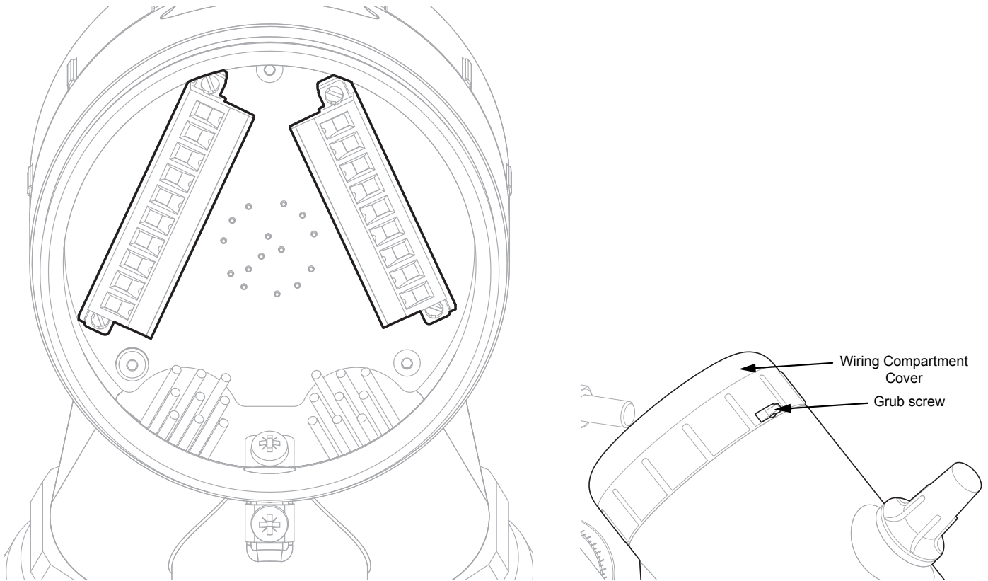
Figure 18. PCB Terminals
