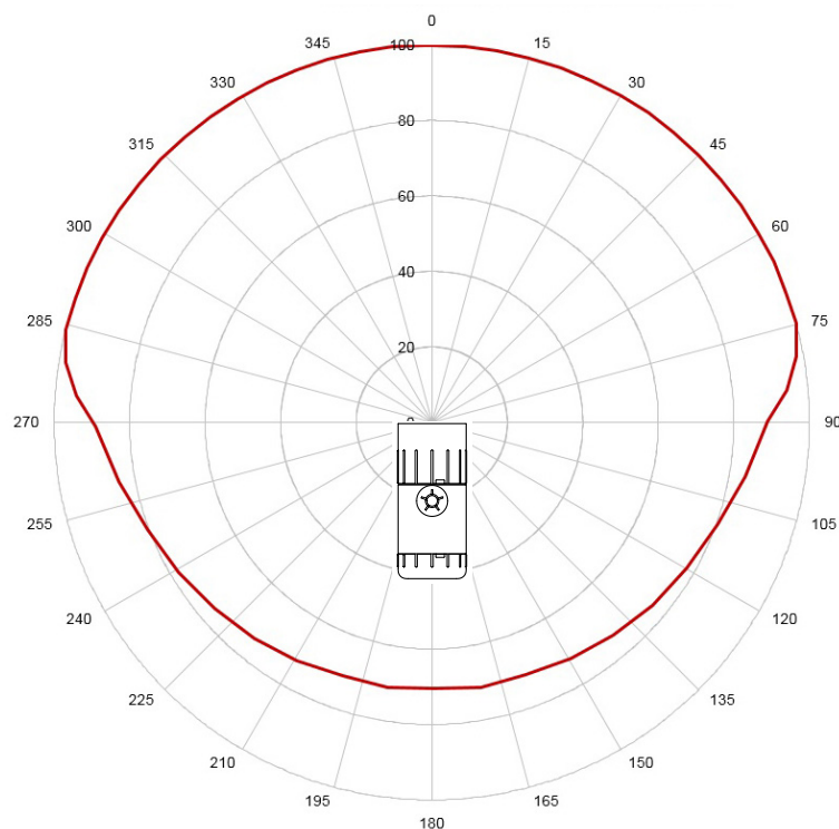
Figure 3. Angular Field of Coverage in Standard Mode (% of Range)
