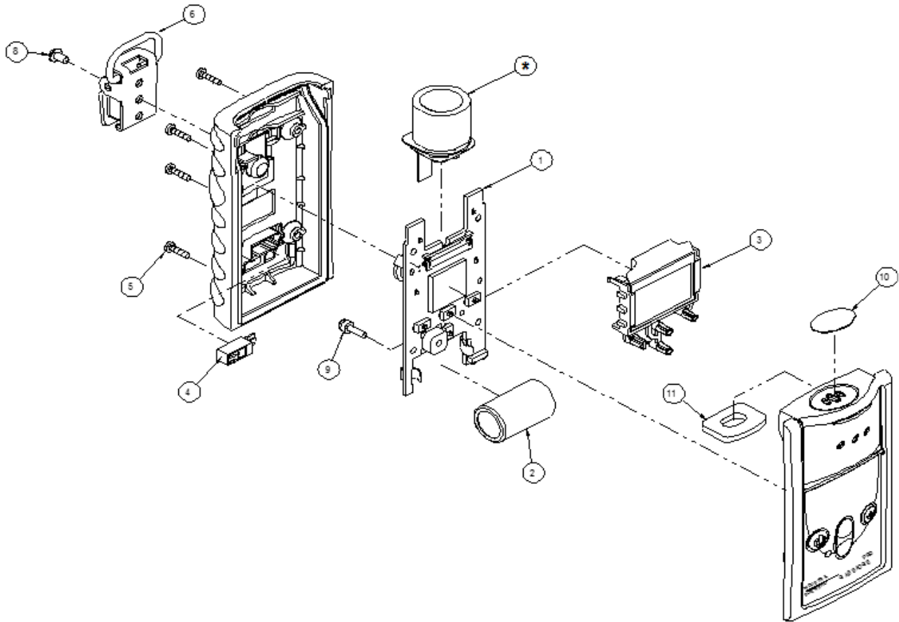
Detailed Components Drawing Showing Replacement Parts
