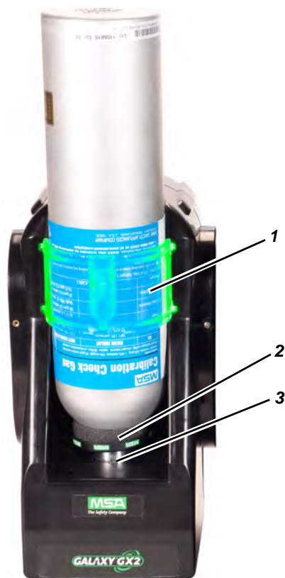
Fig. 7 Cylinder Holder Physical Features
