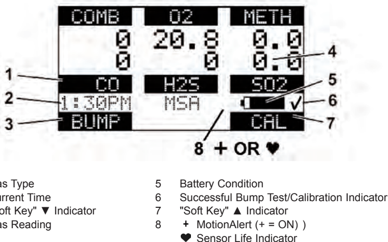
Figure 2-2. Monochrome Display
