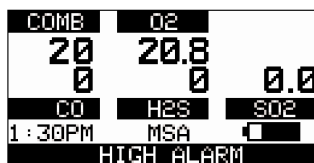
Figure 2-6. Alarm Conditions (High Alarm shown)
