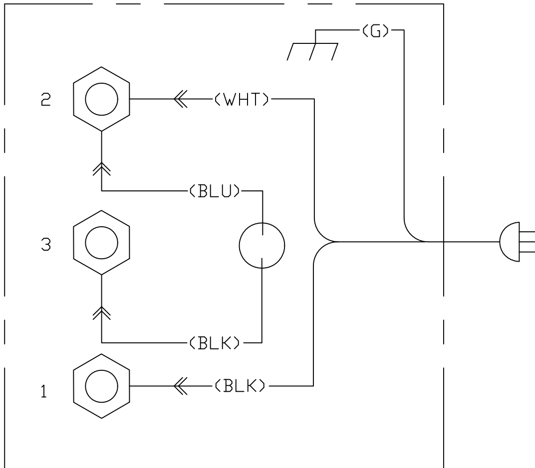
Figure 3.2a: #1000 Wiring Diagram
