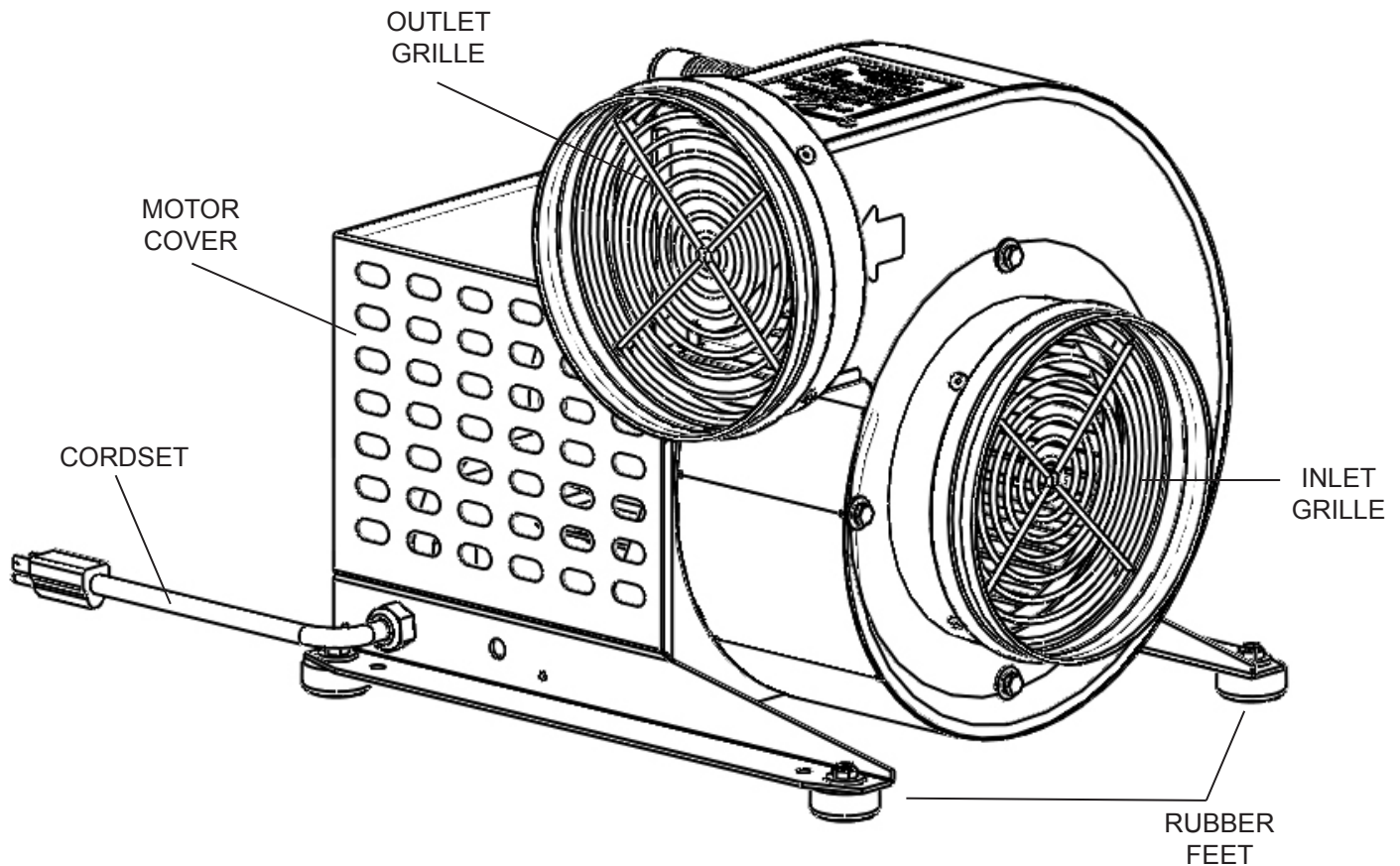
Figure #5.2a: #1000 Centrifugal Blower Pre-Operation Inspection Points
