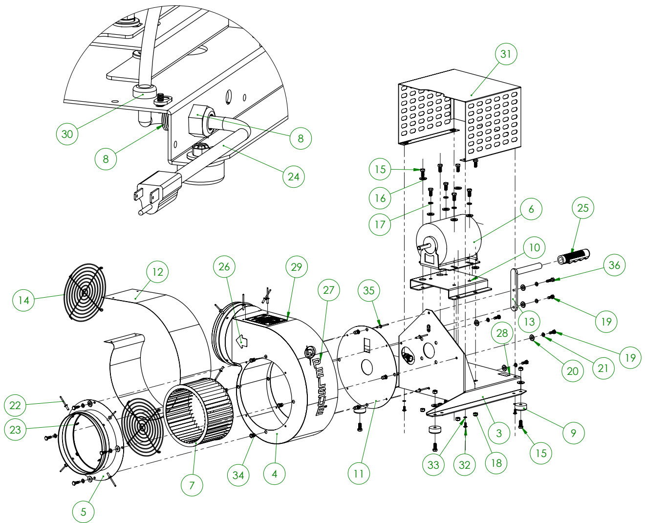
Figure 3.1a: #1000 Parts Diagram
