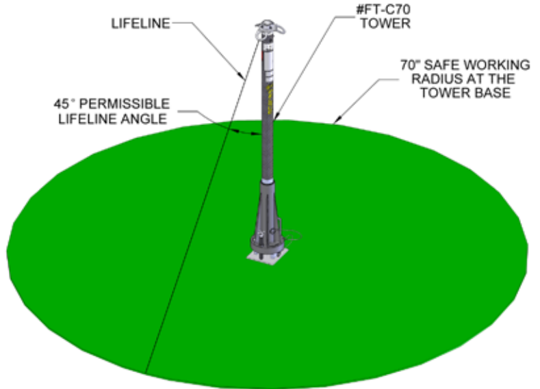
SAFE WORKING RADIUS - MODEL #FT-C70
