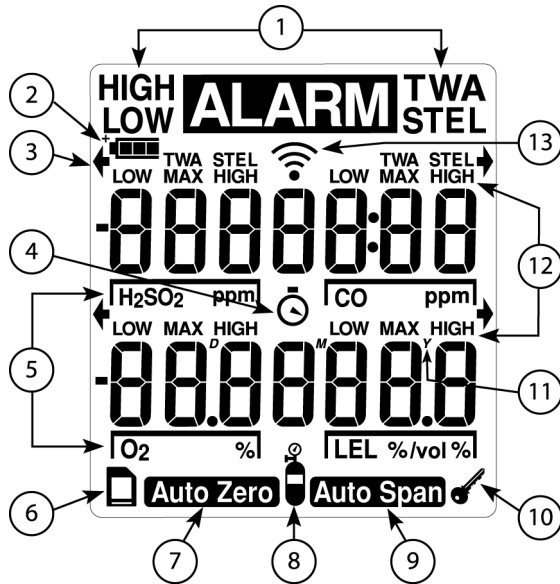
Figure 2. Display Elements
