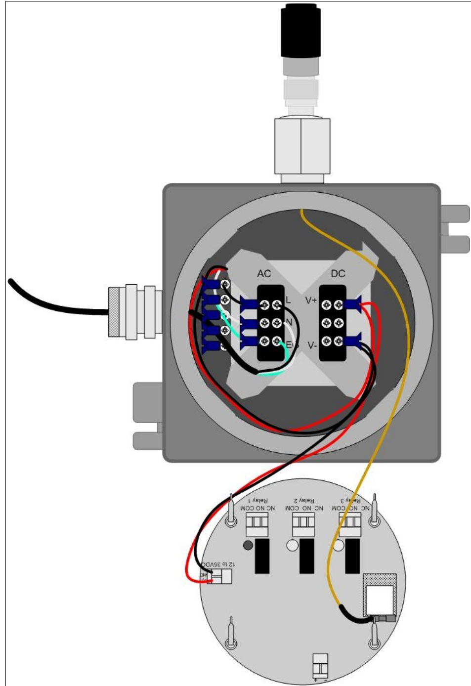
Basic AC Wiring – From Factory:
