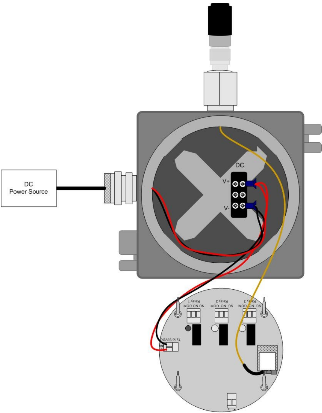
Basic DC Wiring – From Factory:
