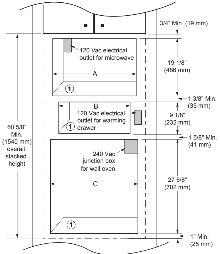
CUTOUT DIMENSIONS DCM24 SHOWN
