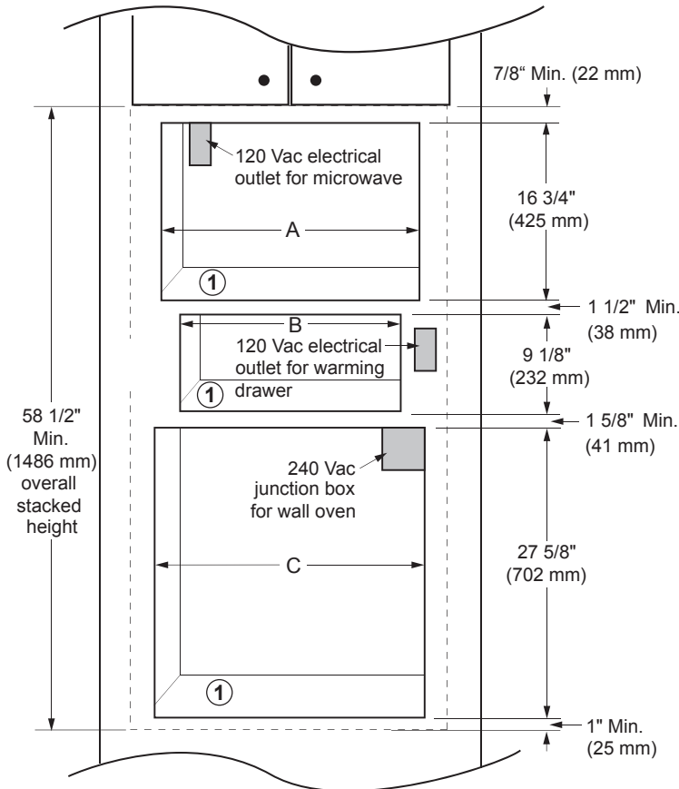
CUTOUT DIMENSIONS DMT2420 SHOWN
