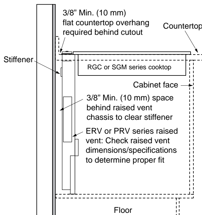
Side View - RGC/SGM Series Cooktop with ERV/PRV Series Raised Vent
