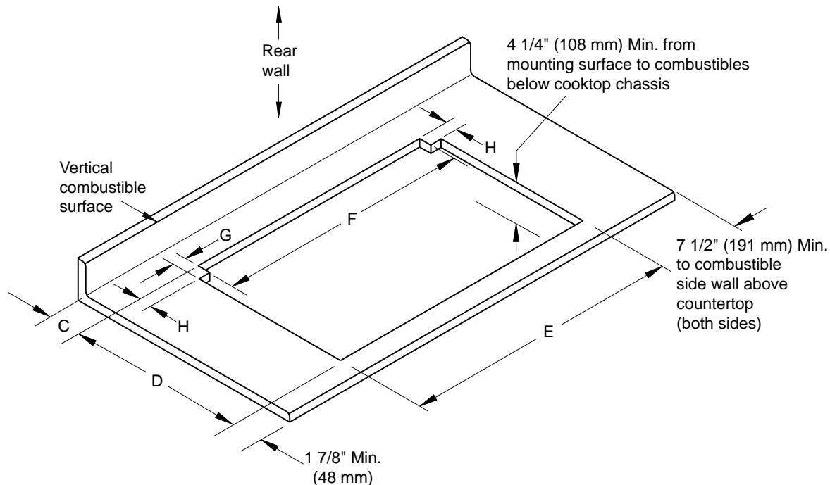
Figure 2 - Notched Countertop Cutout Diagram (SGM466 only)
