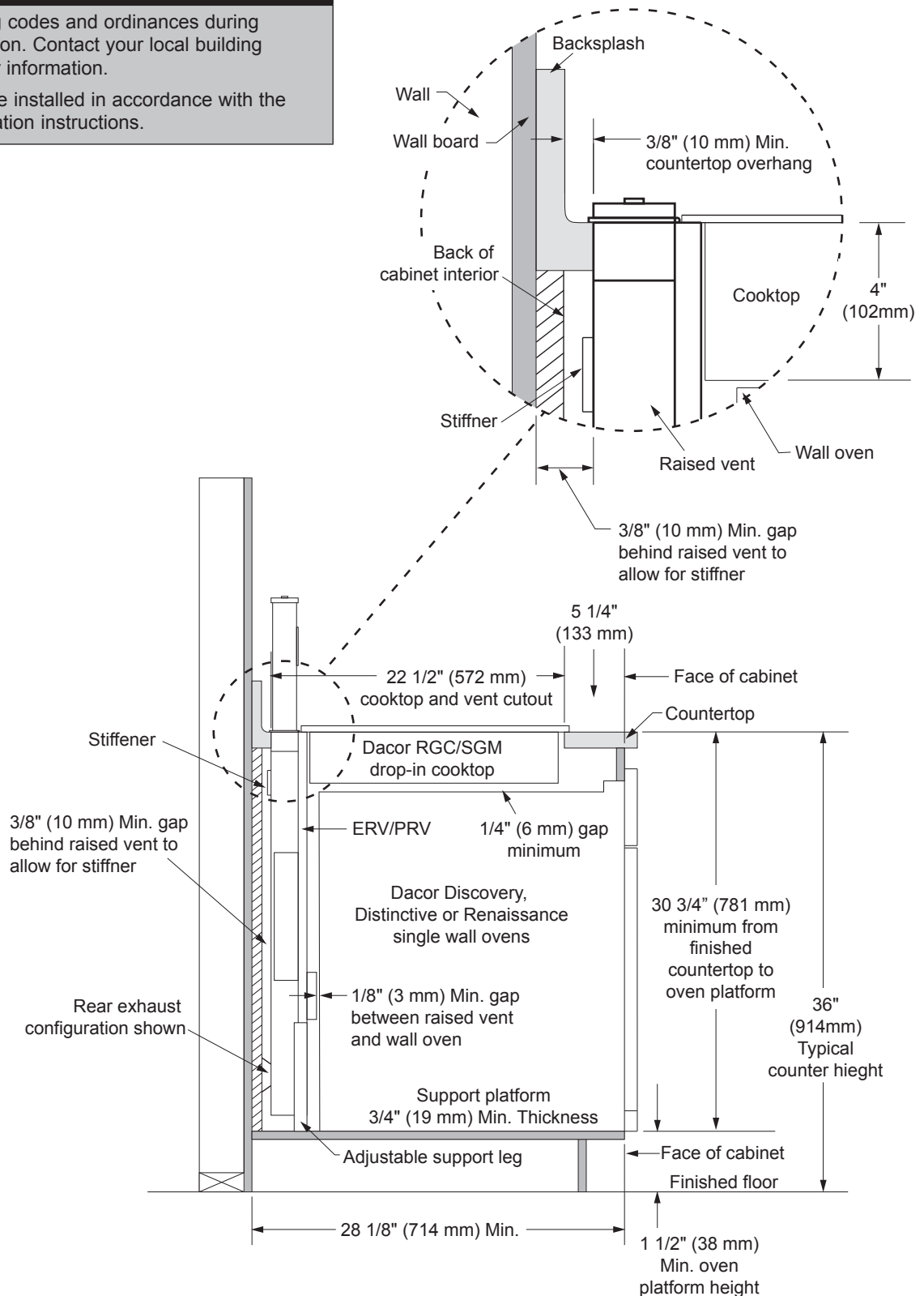
CUTAWAY SIDE VIEW
