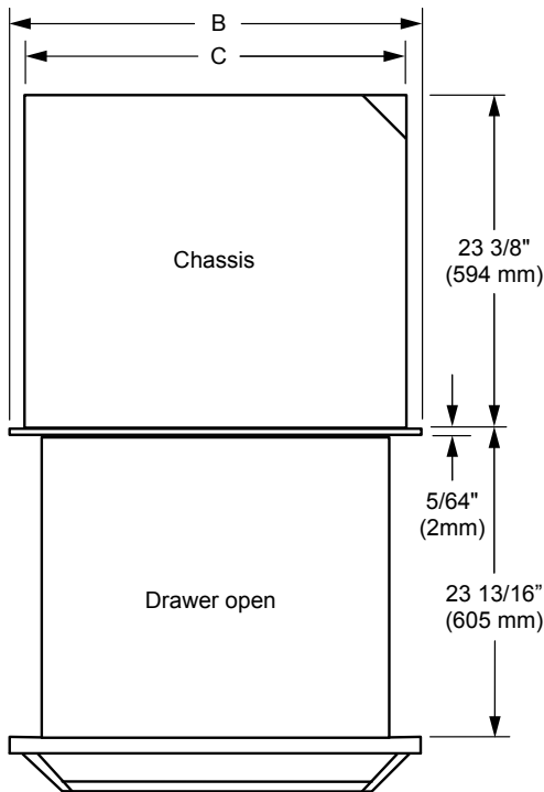
OVERALL DIMENSIONS - TOP VIEW (EWD SERIES SHOWN)
