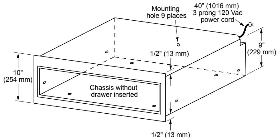
CHASSIS DIMENSIONS
