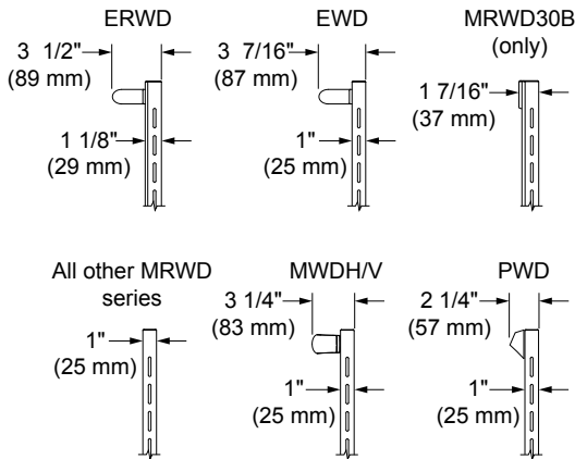
HANDLE DIMENSIONS - SIDE VIEW
