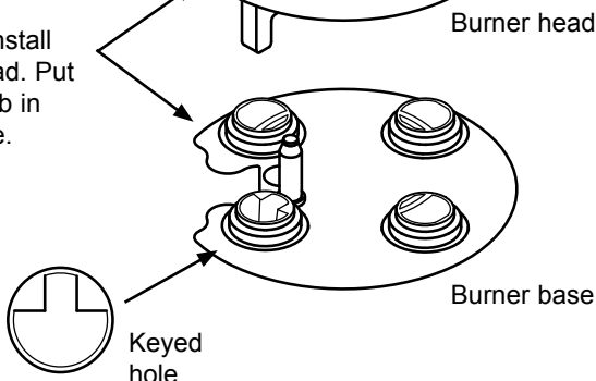
Crown Burner Installation
