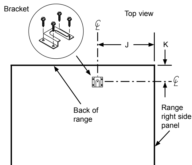
ANTI-TIP BRACKET PLACEMENT
