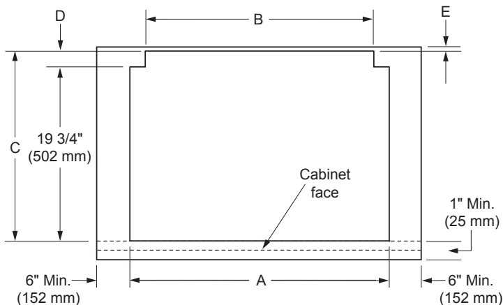
COUNTERTOP CUTOUT (WITH RAISED VENT) TOP VIEW
