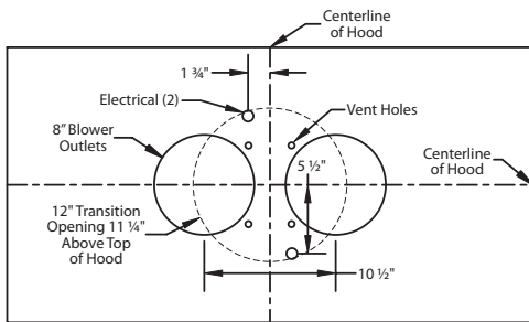
1100 CFM T400 Cluster Blower (Top View)
